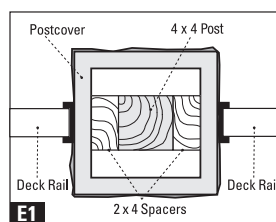
In-line Rail
