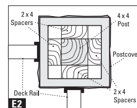
Corner Rail
